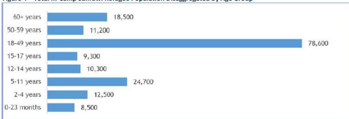
Figure 4 – Total In-Camp Sahrawi Refugee Population Disaggregated by Age Group
