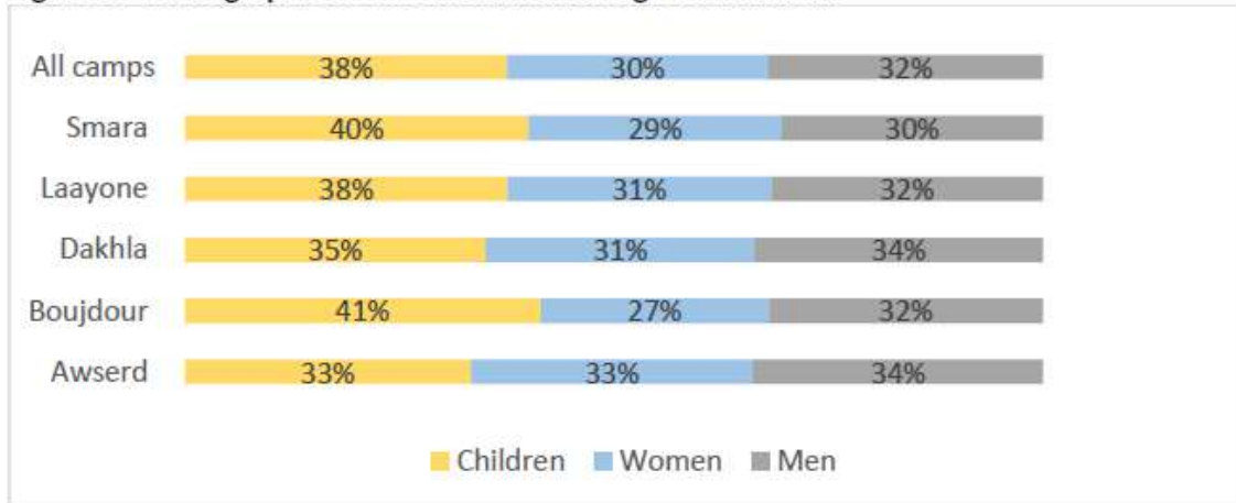
Figure 2 – Demographic Profile of Sahrawi Refugees in Tindouf
